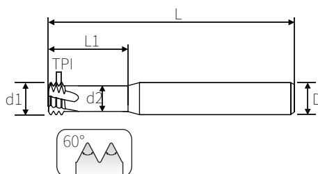
UNF American three-tooth thread milling cutter
